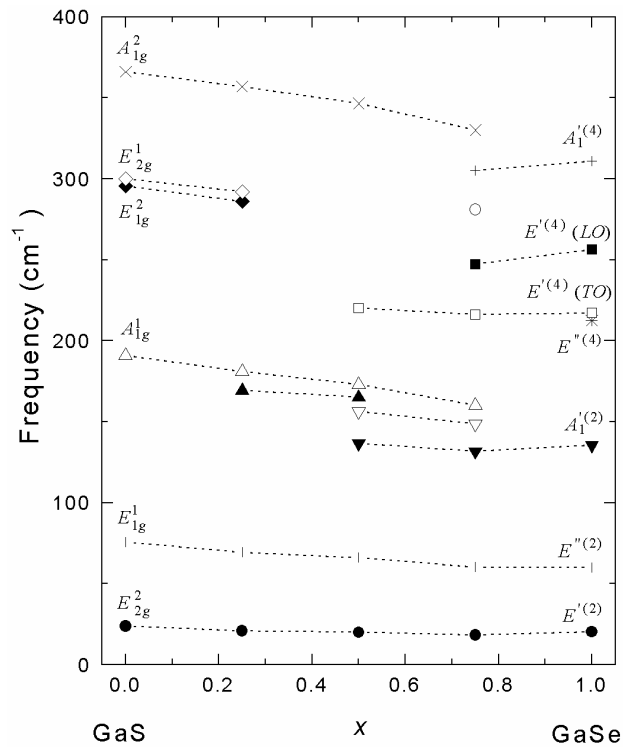
Fig. 5: Frequency dependencies of Raman-active modes on composition of \text{GaSe}_x\text{S}_{1-x} mixed crystals.
