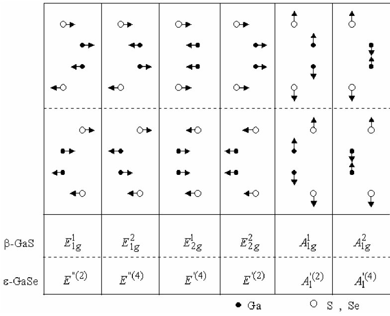
Fig. 2: Atomic displacement vectors for interlayer and intralayer Raman-active optical modes of \beta -GaS and \epsilon -GaSe layered crystals.
