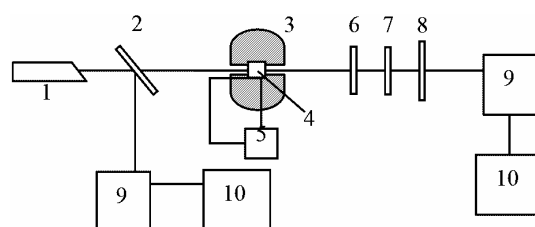
Fig. 2 Experimental setup for SHG measurement. 1: Laser, 2: Beam splitter, 3: Heater, 4: Sample, 5: Temperature controller, 6: 1.06μm reflective mirror, 7: Green glass, 8: 0.53μm interference light filter, 9: Energy detector, 10: Galvanometer.
